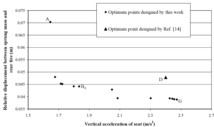
Fig. 6. Pareto front for vertical acceleration of seat and relative displacement between sprung mass and rear tire in 2-objective optimization
